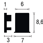
601T004CF Tappi chiusi (opzionale) Closed terminals (optional) Verschlüsse (optional)
